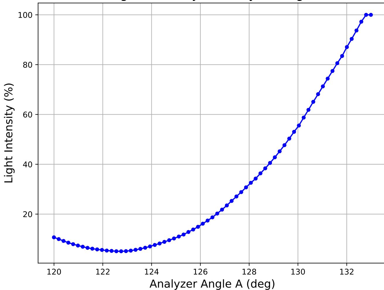
Light Intensity vs Analyzer Angle
